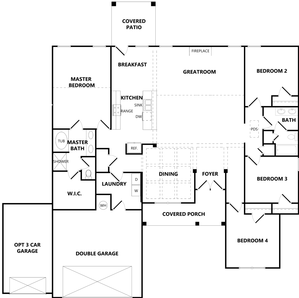
FIRST FLOOR
