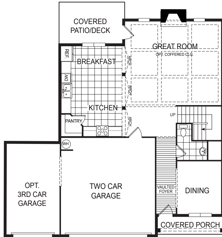
MAIN LEVEL
