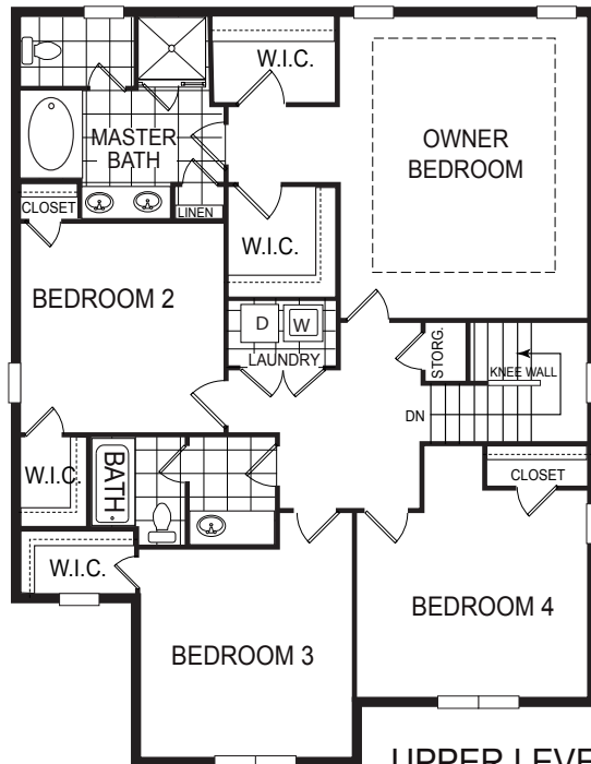
UPPER LEVEL
