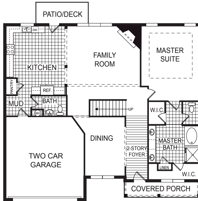
MAIN LEVEL
