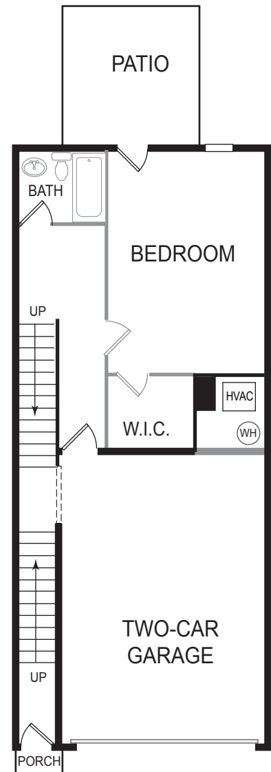
TERRACE PLAN
